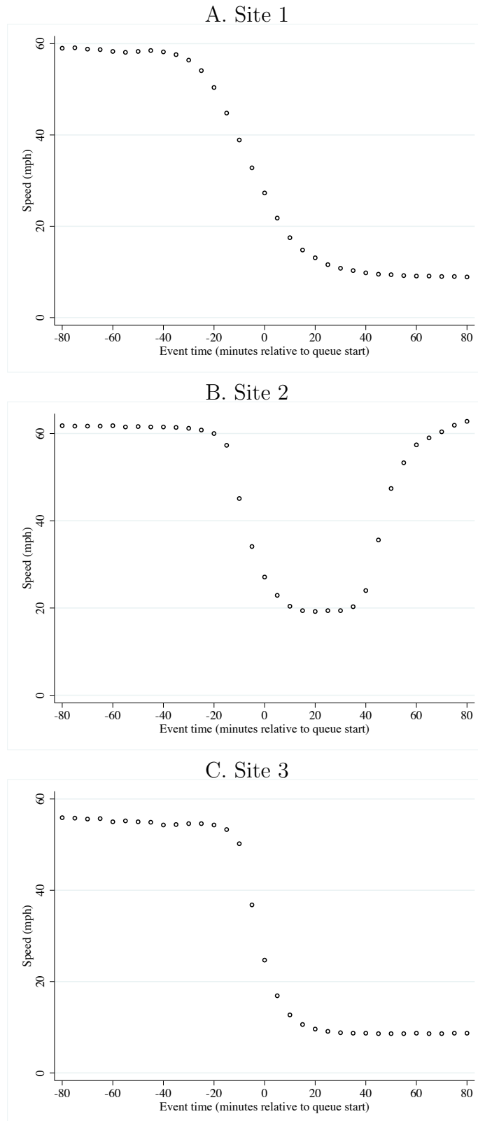
Figure 6: Median Vehicle Speeds at Queue Onset
