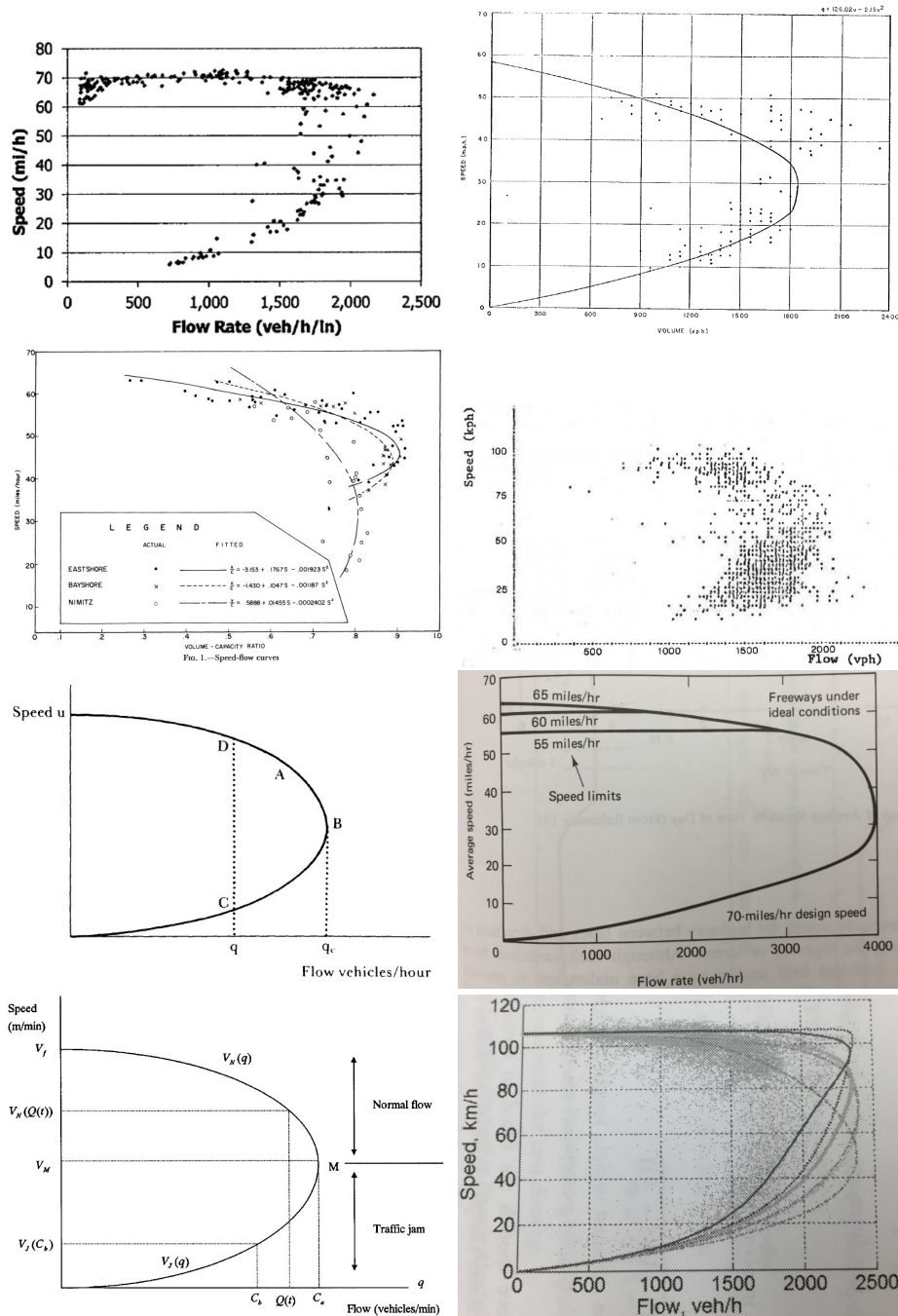
Figure 9: Speed-Flow Curves
